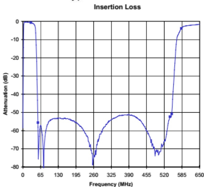
FBR-2/78 Response/ Return Loss Typical Plots
