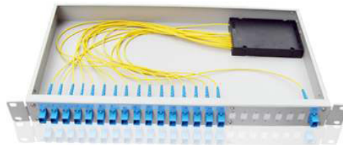
Wiring methods
